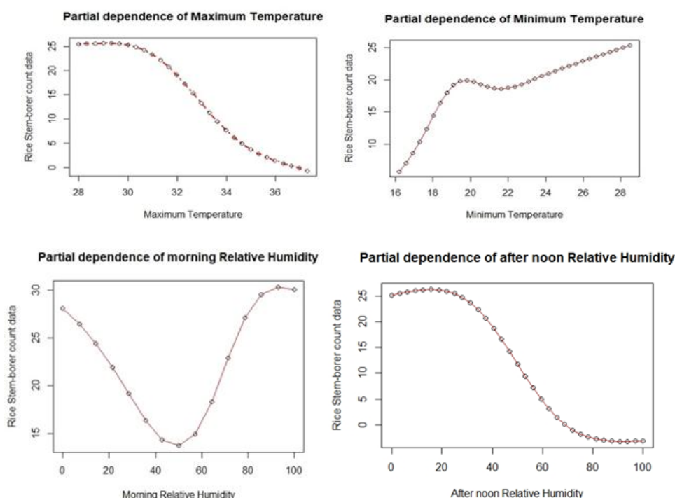
Fig. 6.7 Partial dependence of the input variables of the ANN model
