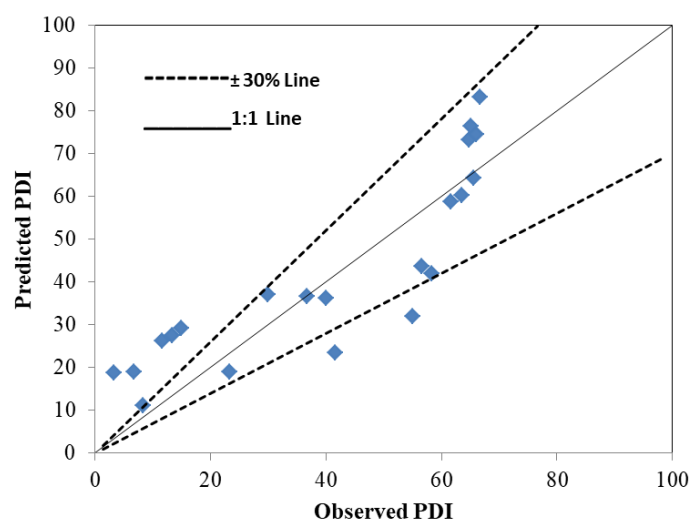
Fig 6.4: Scatter plot of observed vs predicted PDI to validate the model for the year 2022
