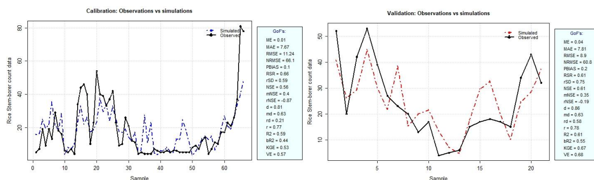
Fig. 6.6 Visualization of calibration and validation of the ANN model
