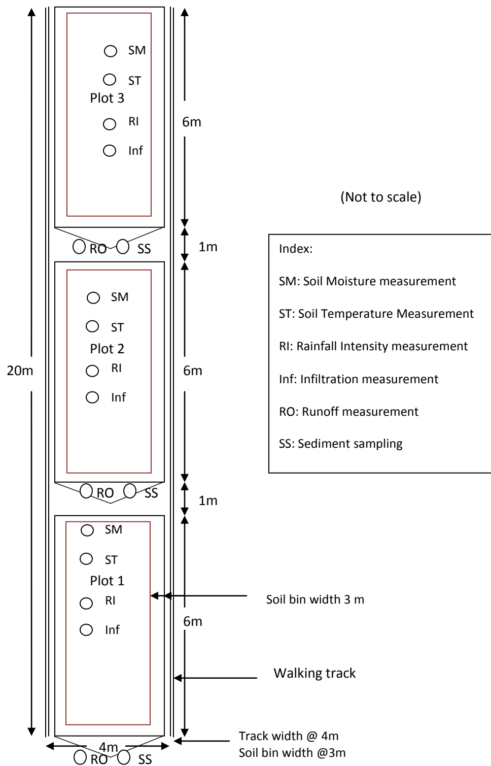
Fig 2. Experimental Lay out of the Rainfall simulator (Modified figure)
