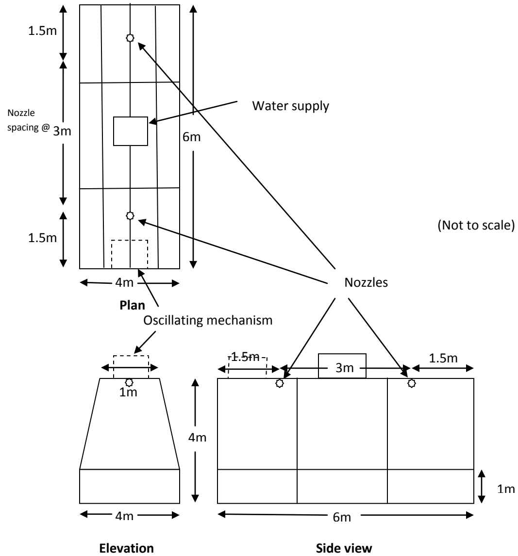
Fig1. Drawing of rainfall simulator (Modified figure)
