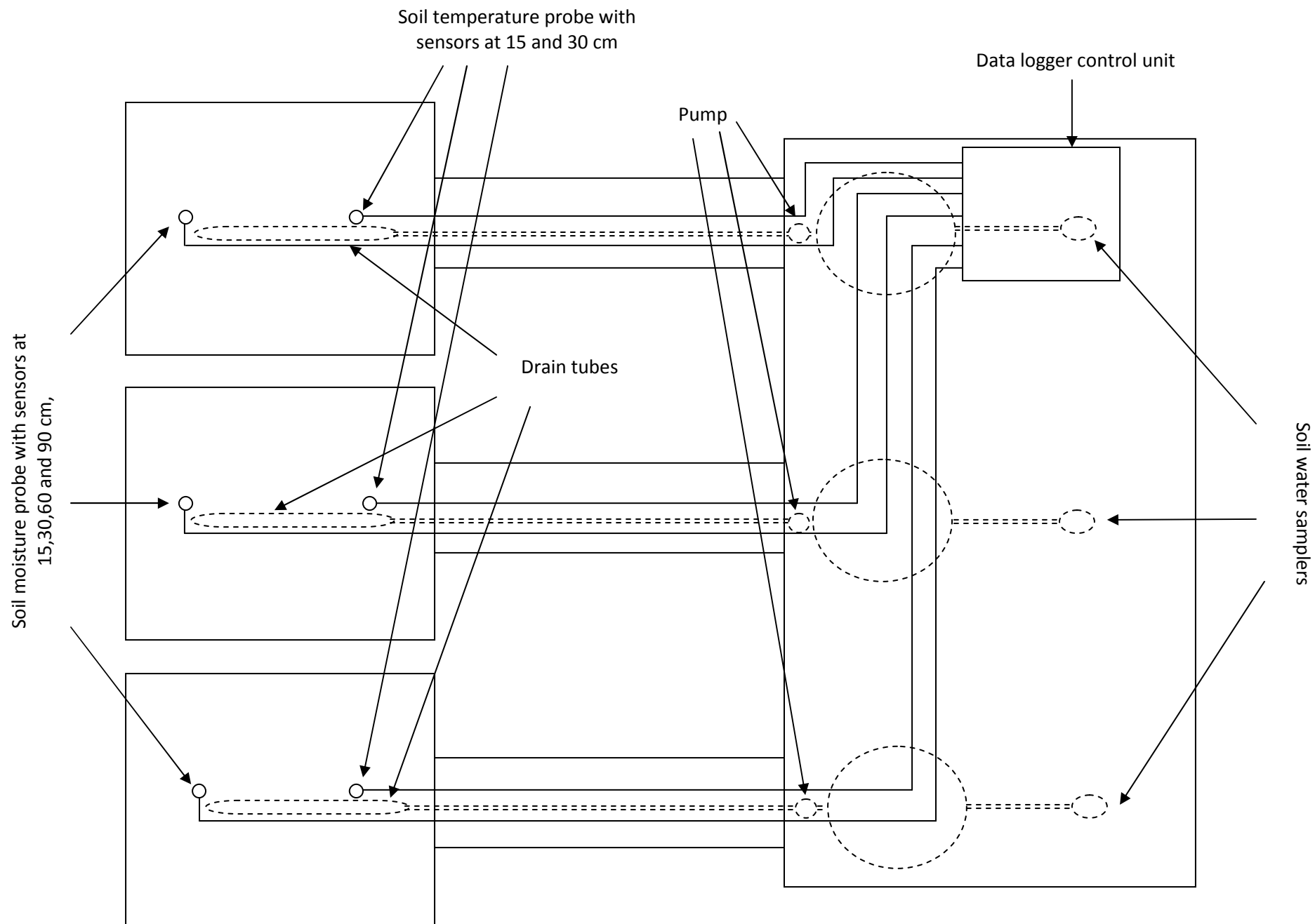
Fig. 2: Experimental Layout of the Lysimeter setup with control room (For example)
