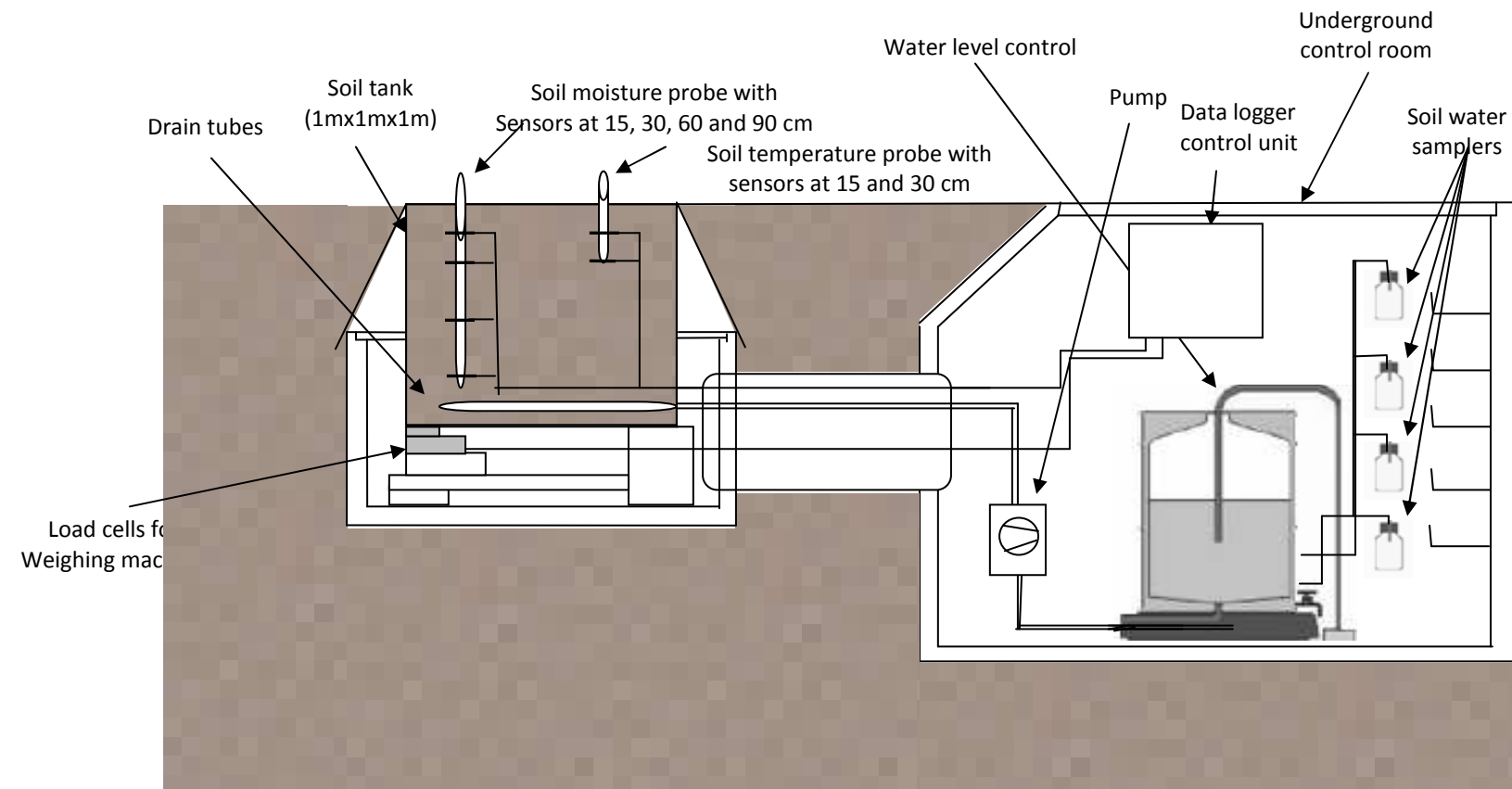
Fig. 1: Schematic diagram of the Lysimeter
